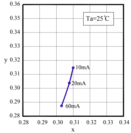
● Forward Current vs. Chromaticity Coordinate
